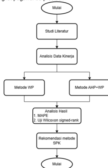
Gambar 1. Metode Penelitian
