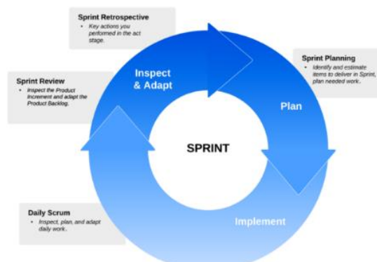
Gambar 1. Metode SCRUM [12]
